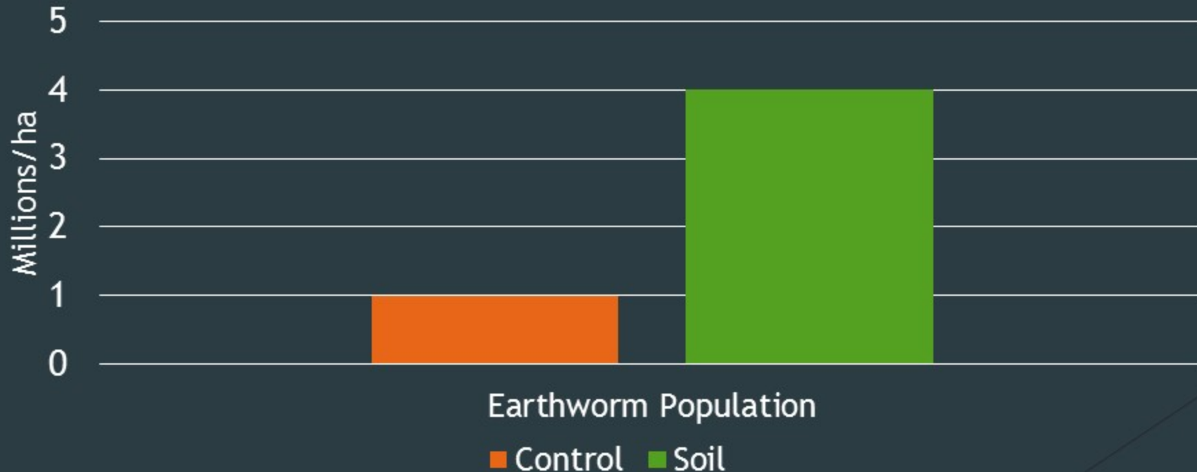
Earthworm population under kiwifruit orchard
